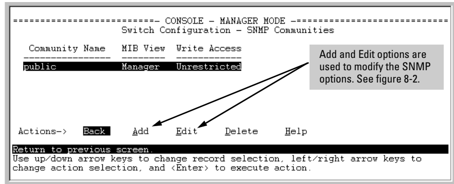
Figure 12-5. The SNMP Communities Screen (Default Values)
