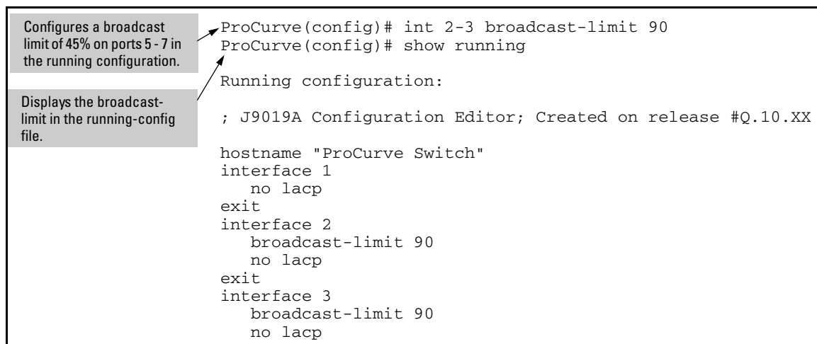
Figure 10-8. Configuring and Displaying a Per-Port Broadcast Limit on Switch 2510
